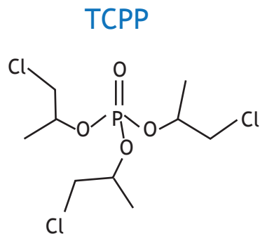
THE SIMILAR CHEMICAL STRUCTURES OF TCEP, TCPP, AND TDCPP
